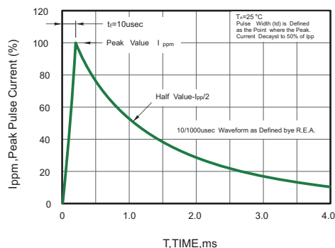
Fig.8 Pulse Waveform
